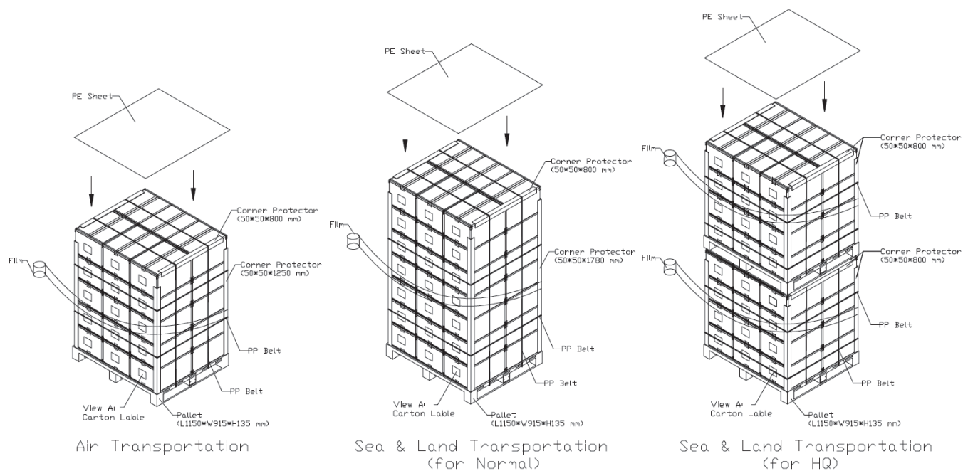
Figure. 7-3 Packing method
