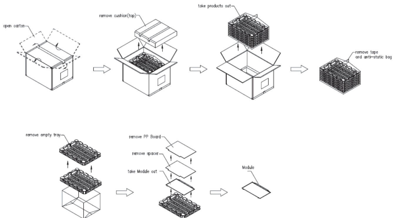
Figure. 7-3 Un-Packing method
