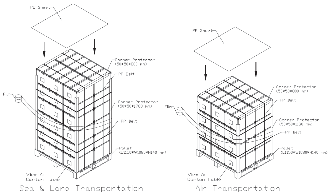
Figure. 7-3 Packing method
