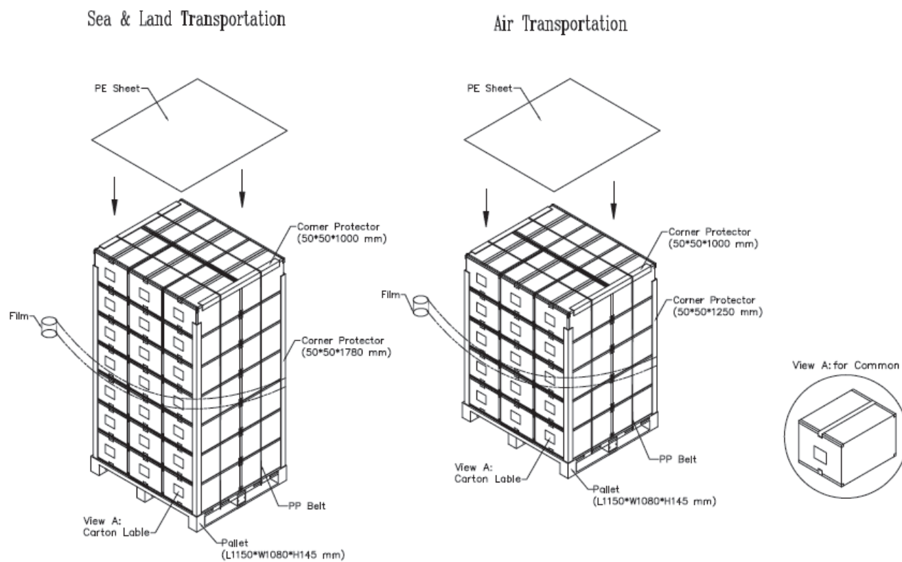
Figure. 7-3 Packing method
